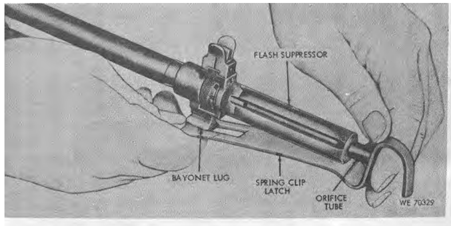
Figure 2-16. Installation/removal of blank ammunition firing attachment.
