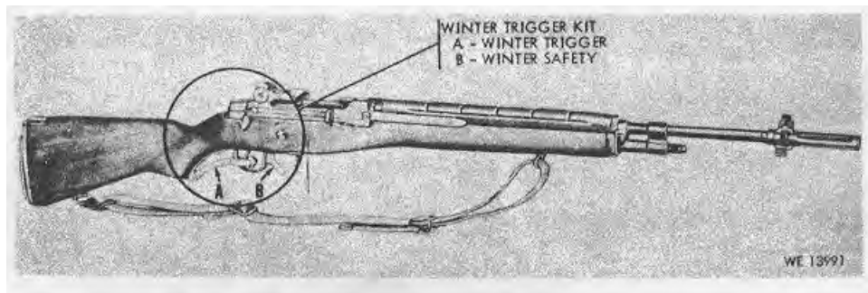
Figure 1-7. 7.62-MM Rifle M14 with winter trigger kit installed.
