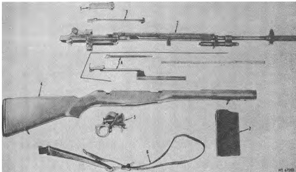
Figure 3-1. Weapon field stripped (M14).
