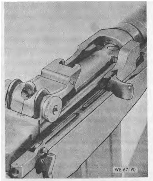
Figure 2-7. Bolt locking and unlocking.
