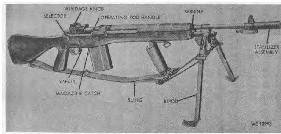
Figure 1-9. 7.62-MM Rifle M14A1-right front view.
