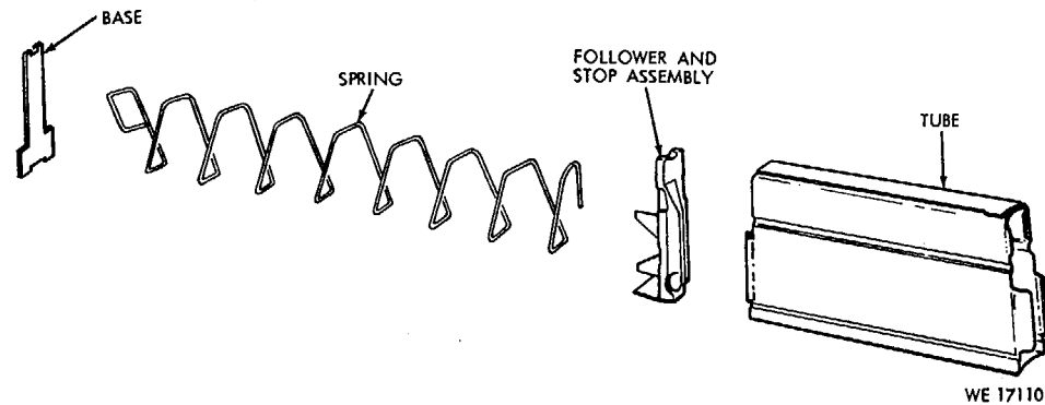
Figure B-1. Magazine-exploded view.
