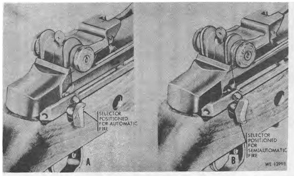
Figure 2-1. Selector set for automatic (A) and semi-automatic (B) fire.
