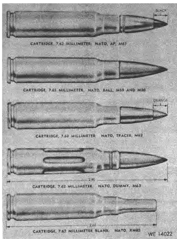
Figure 5-1. 7.62-MM (NATO) cartridges.
