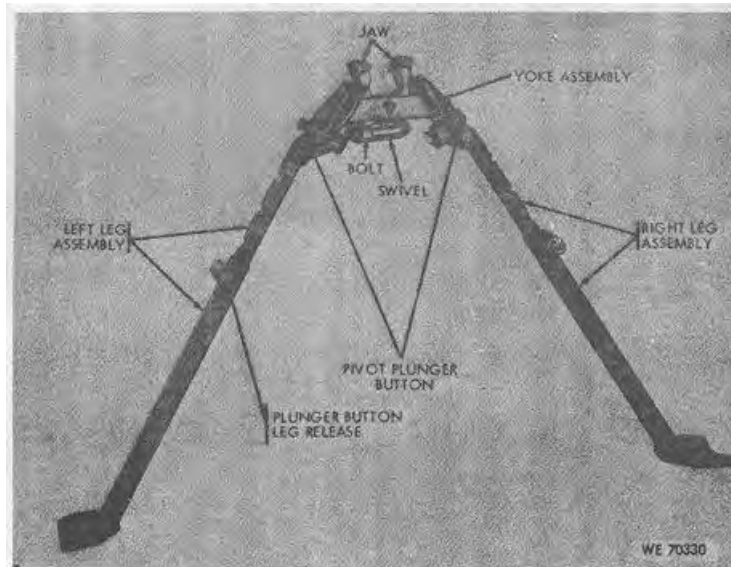
Figure 1-10. Rifle Bipod M2.
