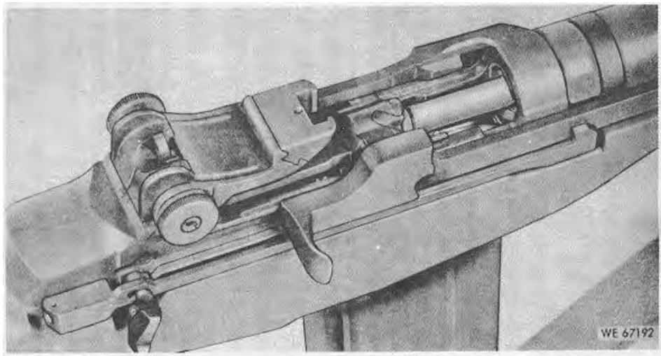
Figure 2-9. Extracting cartridge case from chamber.
