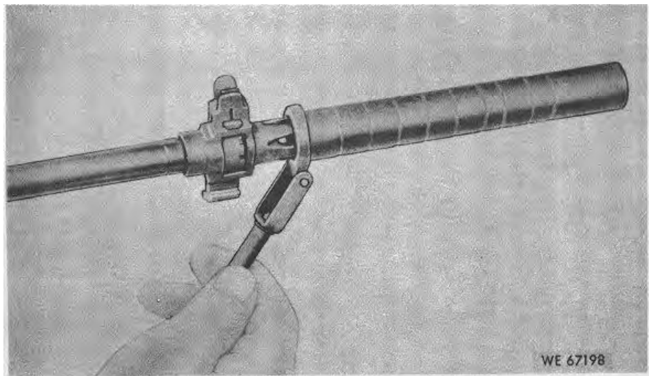
Figure 2-15. Installation/removal of grenade launcher.
