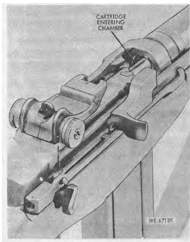
Figure 2-6. Chambering the cartridge.
