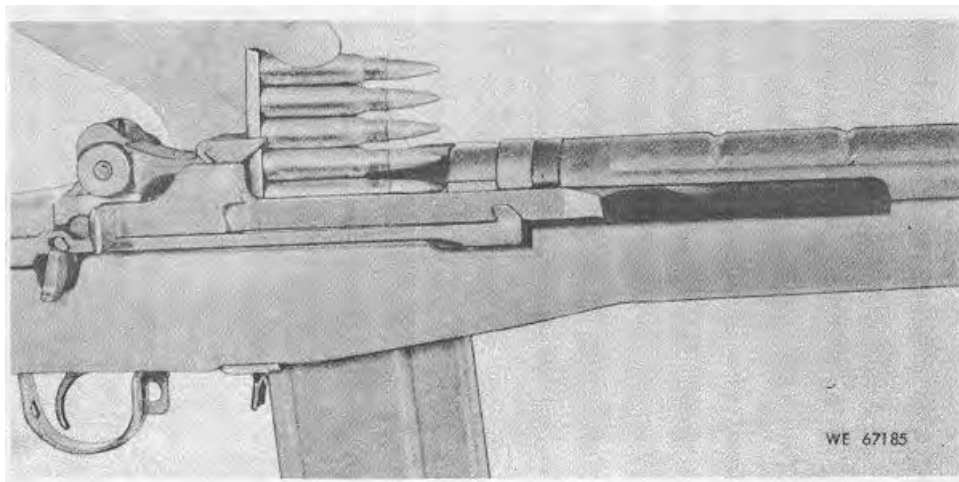
Figure 2-4. Loading magazine with clip.
