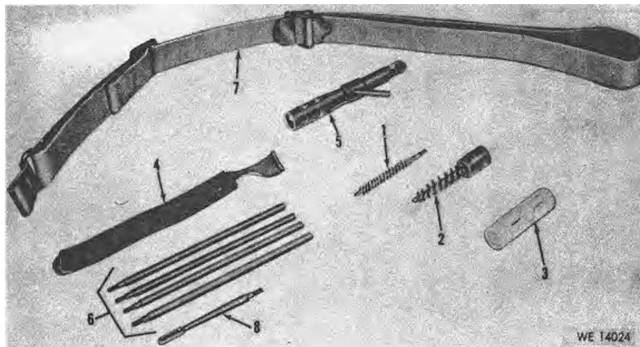
Figure B-2. Tools and equipment.
