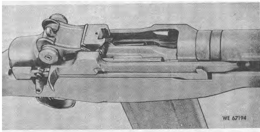
Figure 2-11. Showing bolt in open position.
