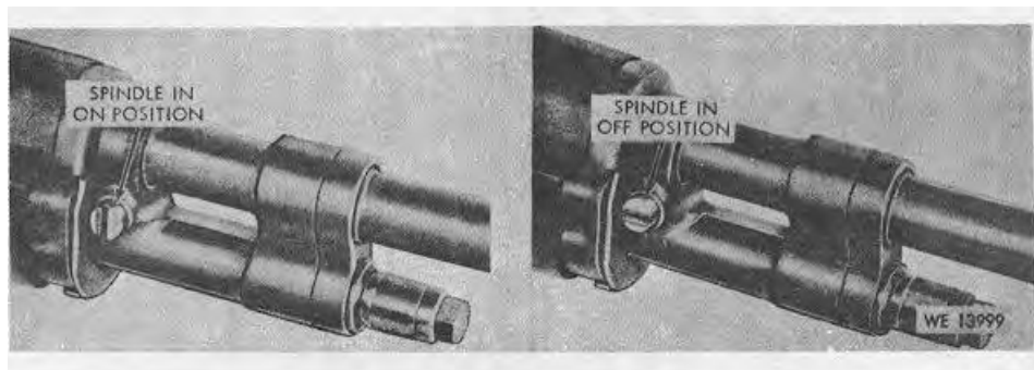
Figure 2-13. ON-OFF position of spindle valve.
