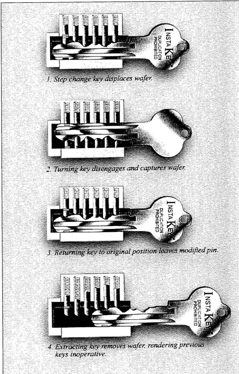
Figure 4-4. InstaKey
