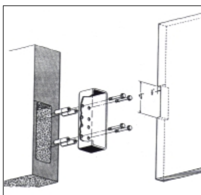
Figure 7-11. Wall mounting box.
