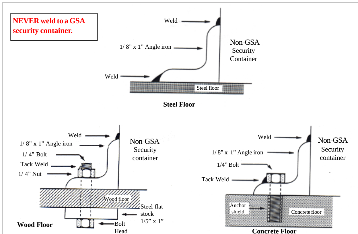
Figure 3-12. Container anchoring methods.
