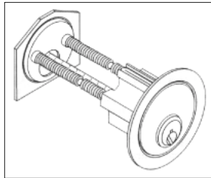
Figure 4-9. Rim cylinder.
