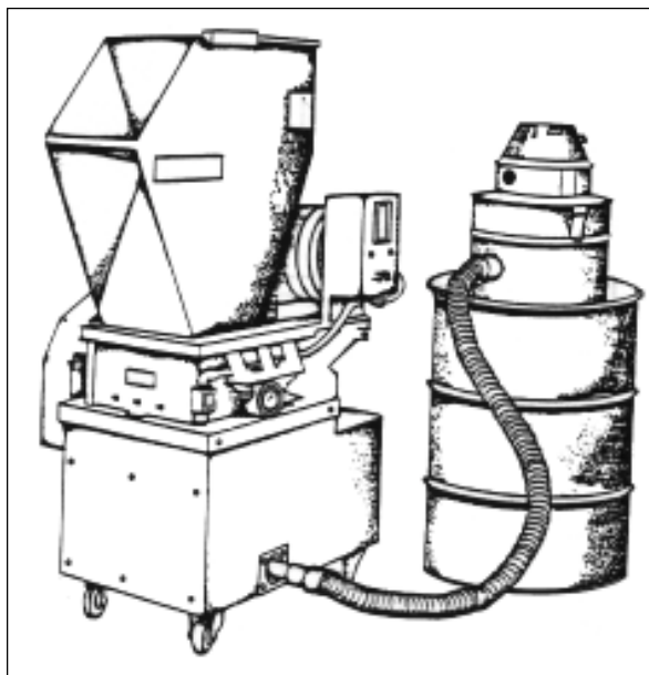
Figure 8-3. Volume shredder.
