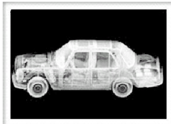
Figure 2-18. Backscatter image of car with cocaine simulant in trunk.
