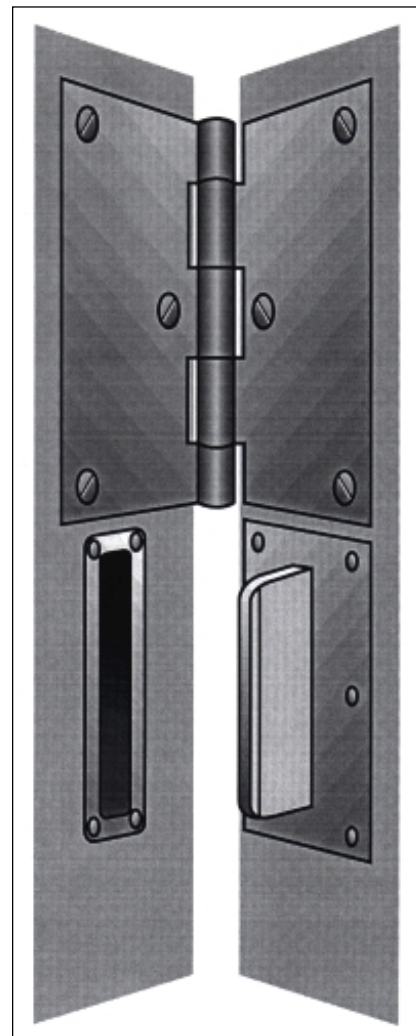
Figure 7-2. Pin-and-socket hinge.
