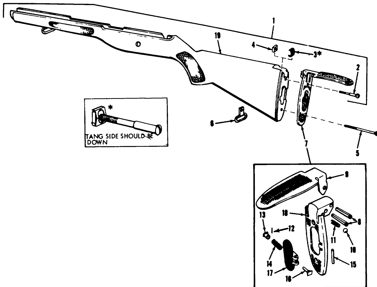
Figure 4. Stock assembly with butt plate, Rifle, M14-exploded view.
