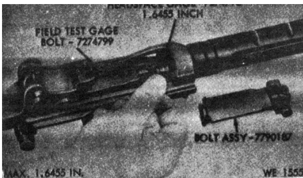
Figure 7-3. Gaging headspace.
