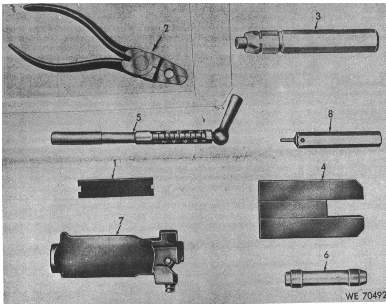
Figure 15. Maintenance Tools.
