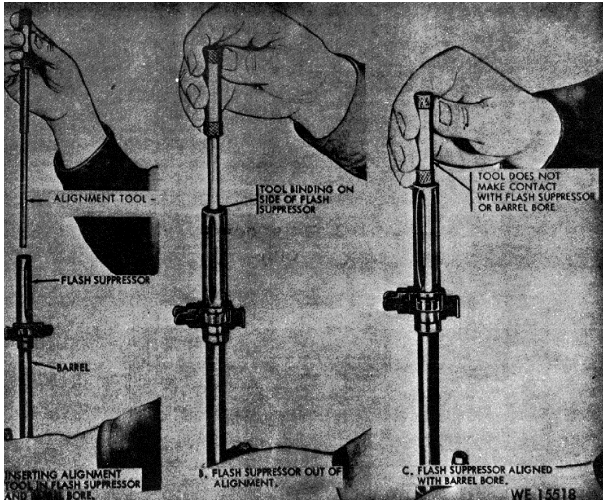
Figure 8-3. Checking alignment of flash suppressor with alignment tool.
