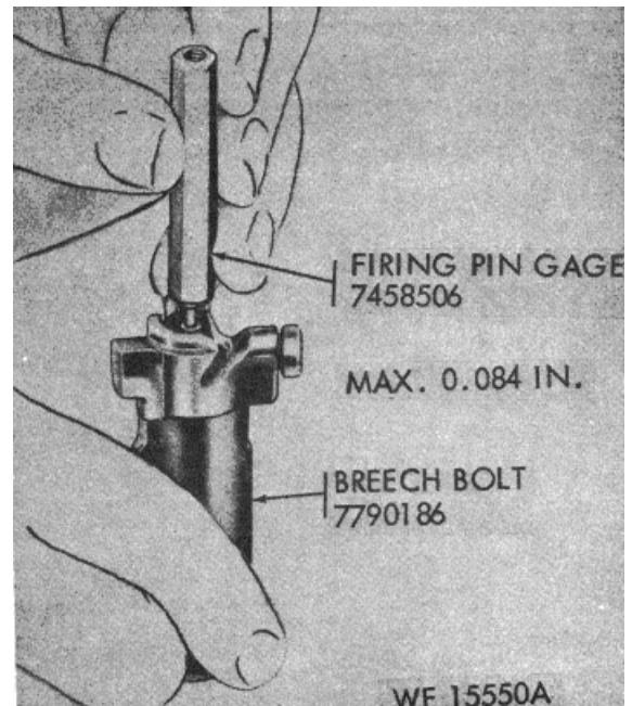
Figure 7-2. Checking diameter of firing pin hole.
