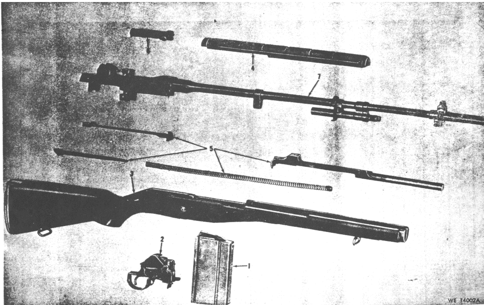
Figure 1. Major groups and assemblies - M14.
