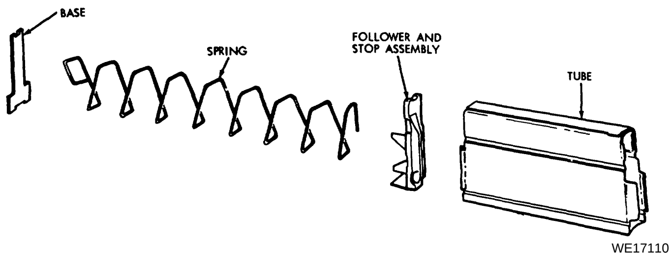
Figure 3-1. Magazine exploded view.
