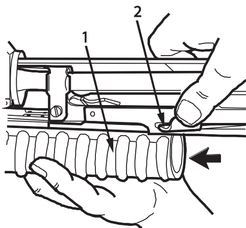
Figure 4. Barrel Latch-Disassembly.
