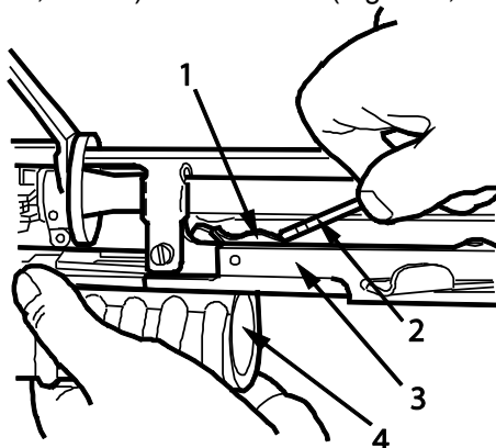
Figure 5. Barrel Stop-Disassembly.
