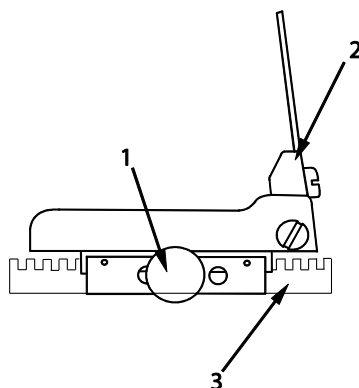
Figure 2. Leaf Sight
