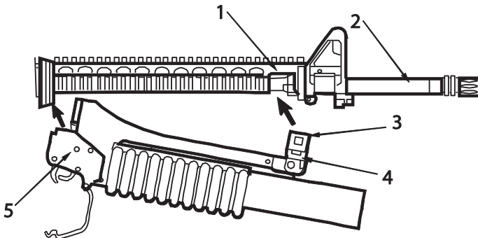
Figure 6. Rifle/QRB Installation.
