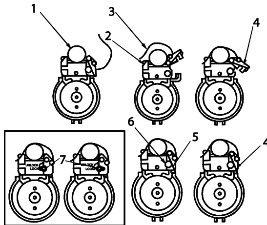
Figure 8 QRB Installation
