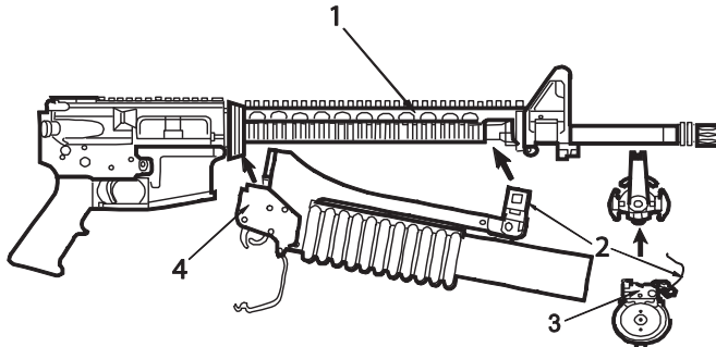
Figure 4. Rifle/QRB Installation.
