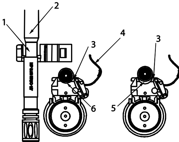
Figure 7. Carbine/QRB Installation.
