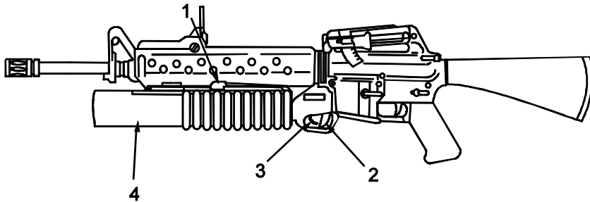
Figure 3. Barrel Latch
