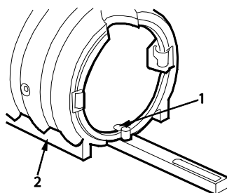
Figure 6. Locator Slot.
