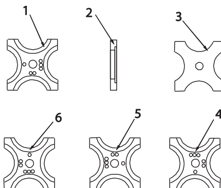
Figure 3. Five Position Shim Plate.
