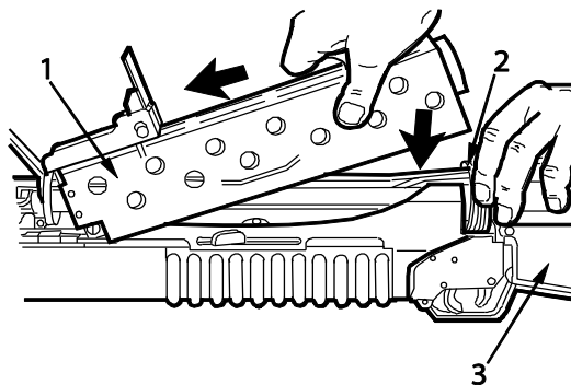
Figure 9. Handguard Leaf Sight-Assembly
