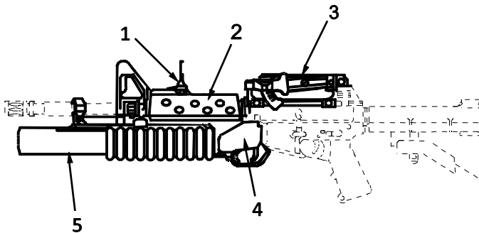
Figure 2. M203A1 Grenade Launcher W/E
