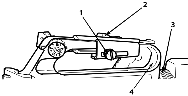
Figure 11. Quadrant Sight-Assembly.
