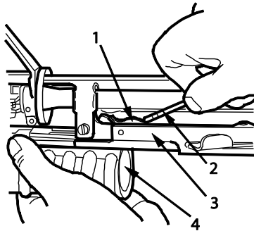
Figure 8. Barrel Stop-Assembly.
